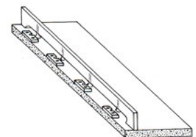
#4 Run a bead of caulk along the line of Smart Clips, and drive the backsplash into position.
